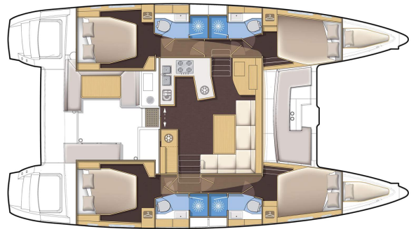
Version 4 cabines / 4 cabin version
