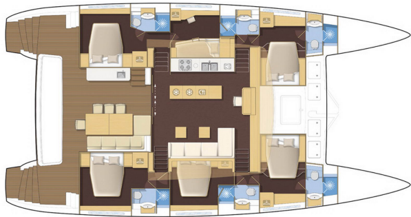
Cuisine centrale, 6 cabines / Central galley, 6 cabin version
